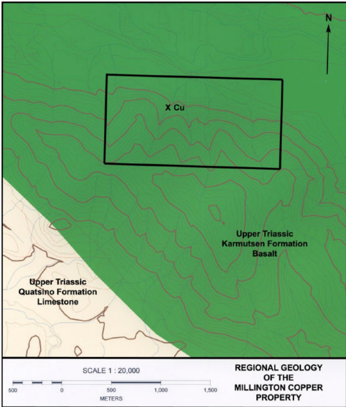
Fig. 4 REGIONAL GEOLOGY OF MILLINGTON COPPER PROPERTY
