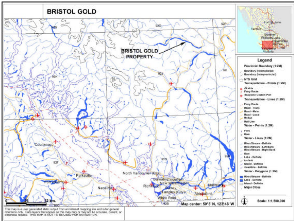
Fig. 1 BRISTOL GOLD PROPERTY BC LOCATION MAP
