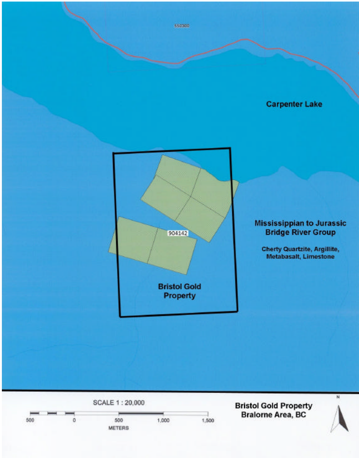
Fig. 4 REGIONAL GEOLOGY OF THE BRISTOL GOLD PROPERTY
