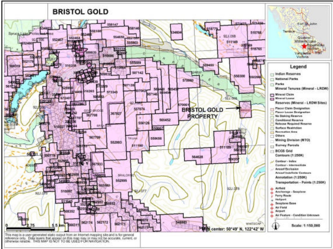
Fig. 2 BRISTOL GOLD PROPERTY REGIONAL LOCATION MAP
