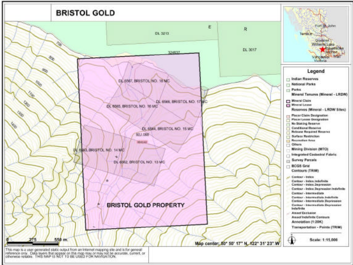
Fig. 3 BRISTOL GOLD PROPERTY MAP
