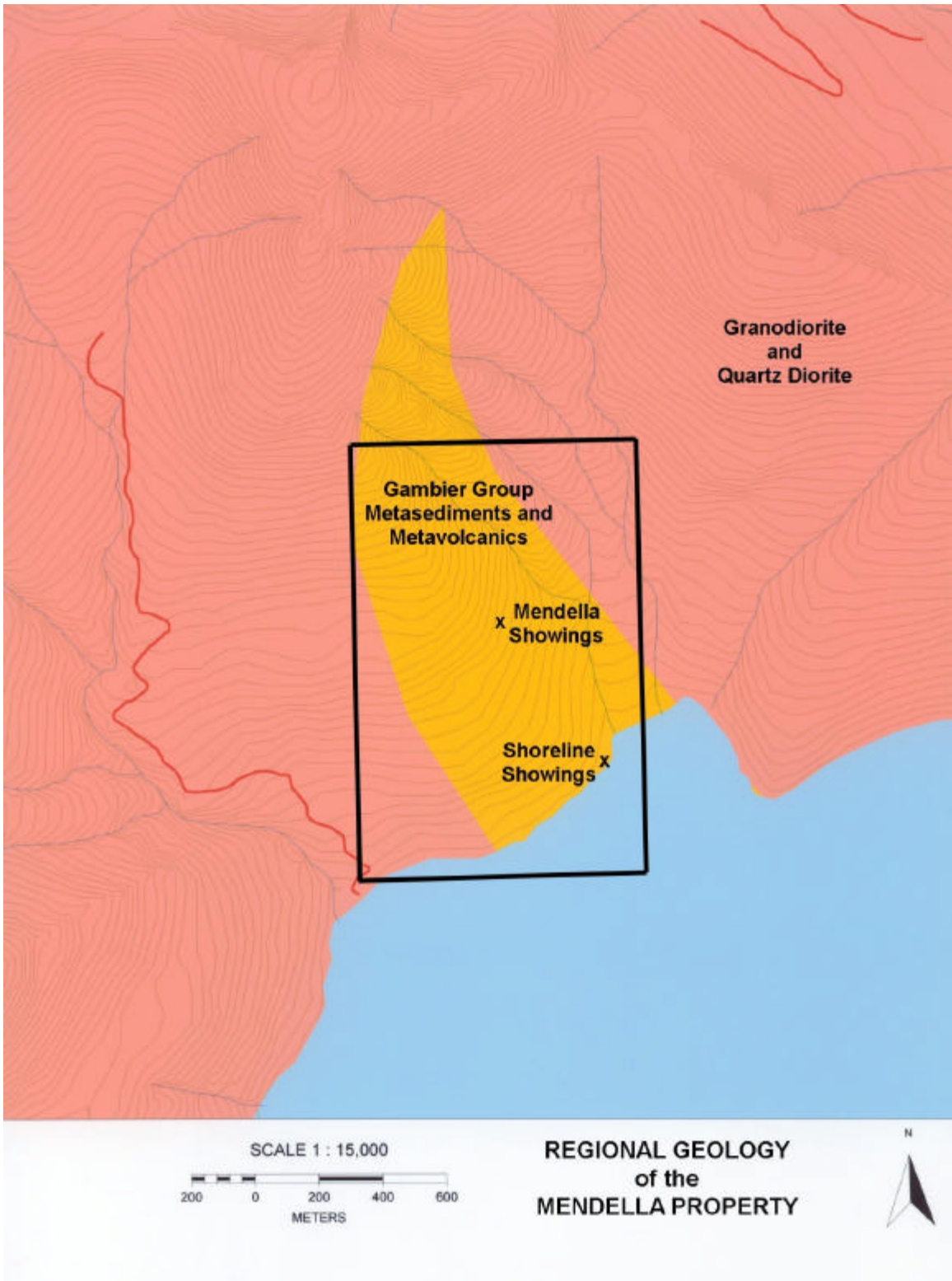
Fig. 4 REGIONAL GEOLOGY OF THE MENDELLA PROPERTY
