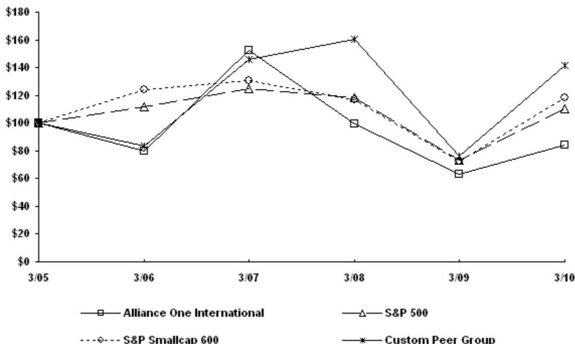
COMPARISON OF 5 YEAR CUMULATIVE TOTAL RETURN 1 Among Alliance One International, the S&P 500 Index, the S&P Smallcap 600 Index and a Peer Group
